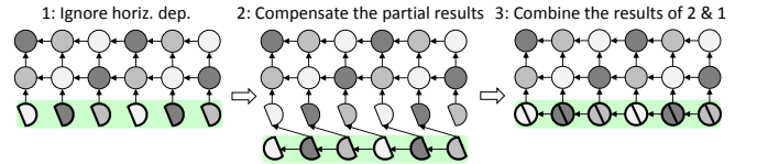
Figure 4: Compensation-based solutions decompose the processing into three steps, each of which can be parallelism-friendly and load balanced.
