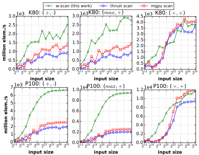
Figure 8: Throughput comparison of the weighted scan kernels.
