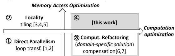
Figure 1: Parallelization landscape for wavefront loops.
