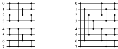
(a) sorting networks (b) merging network
