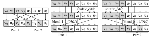
(a) sym-blend (b) sym-blend(details) Figure 10: Symmetric blend operation and its pairing details
