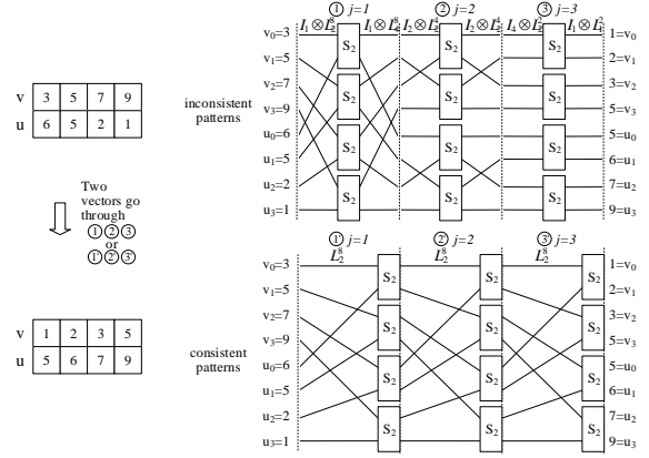
Figure 8: Two formalized variants of bitonic merging networks: the inconsistent pattern and the consistent pattern. All elements in vector v and u are sorted, but inverted in vector u .
