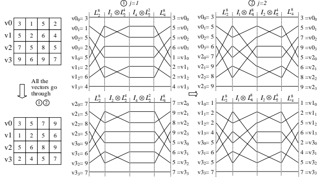
Figure 7: Four 4-element vectors transpose with the formalized permutation operators of DSL.
